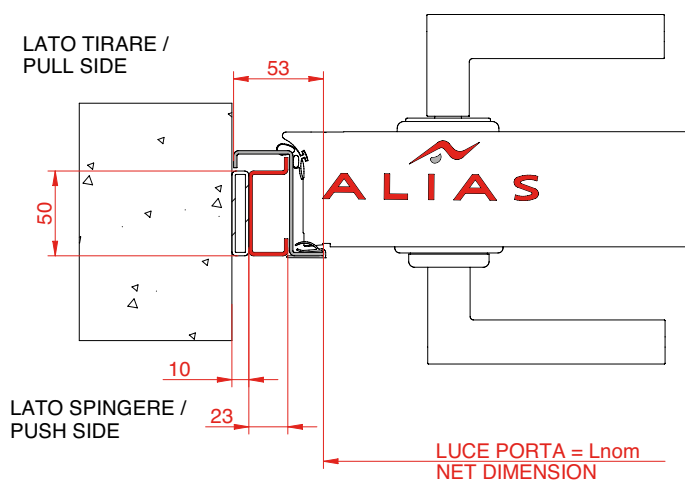
MONTAGGIO IN LUCE Outside wall configuration
