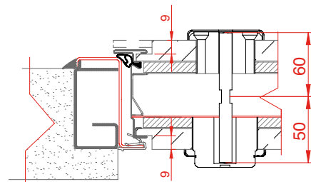
Pantografato 15mm a sporgere - copricarena / 15mm thickness panels that comes out from perimetral profiles
