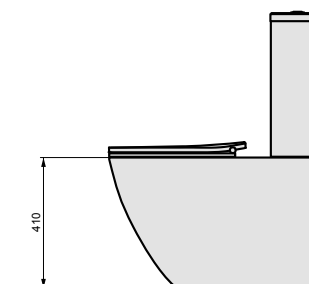
Wc monoblocco Like con cassetta Wc monoblock Like with cistern Bidet Like a terra Bidet Like back to wall
