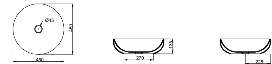
cod. EALAVRO45 Lavabo Easy Tondo Ø45 Easy washbasin Round Ø45
